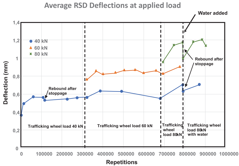
Figure 6. Average surface deflections measured with the RSD.
