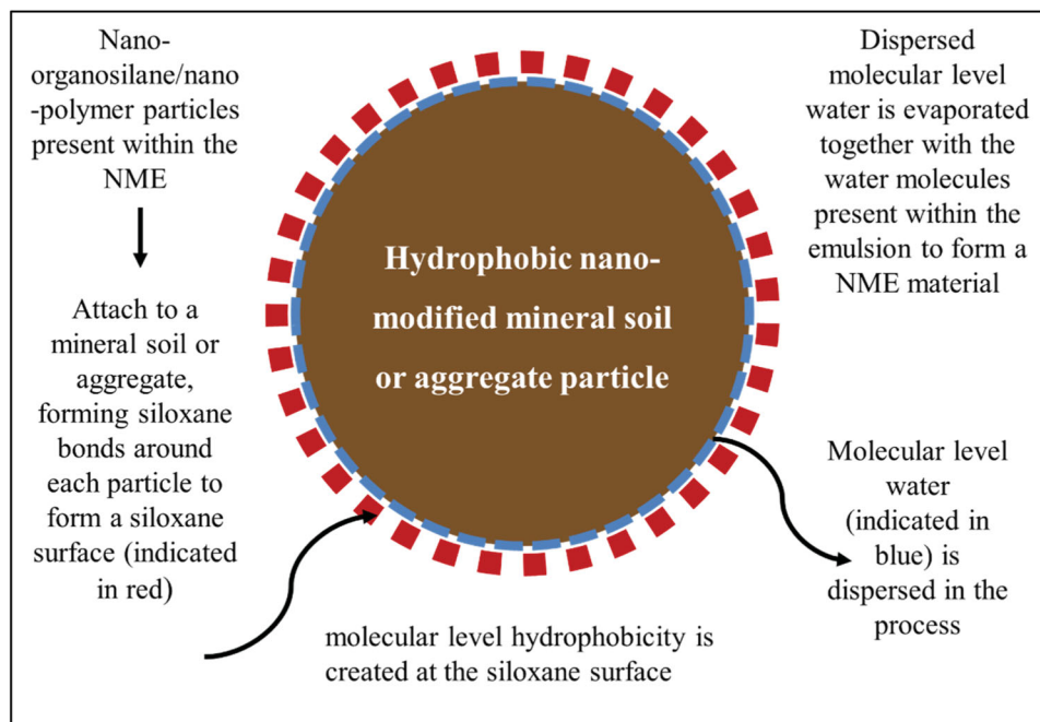
Figure 1. Summary of the formulation of a siloxane surface on a NME stabilised mineral soil or aggregate (Akhilwaya and Rust, 2018).
